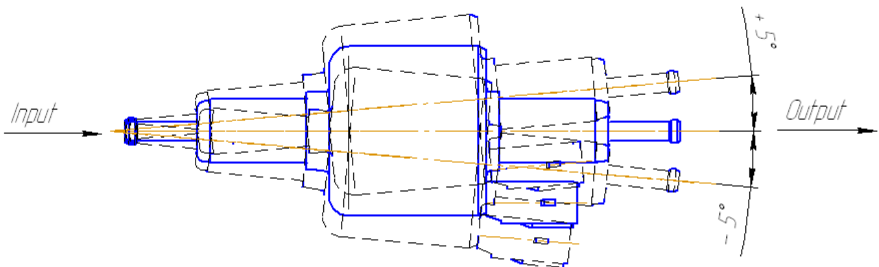
Figure 7.7 - Permissible mounting position of fuel supply pump (for petrol fuel pump production Thomas Magnete).
