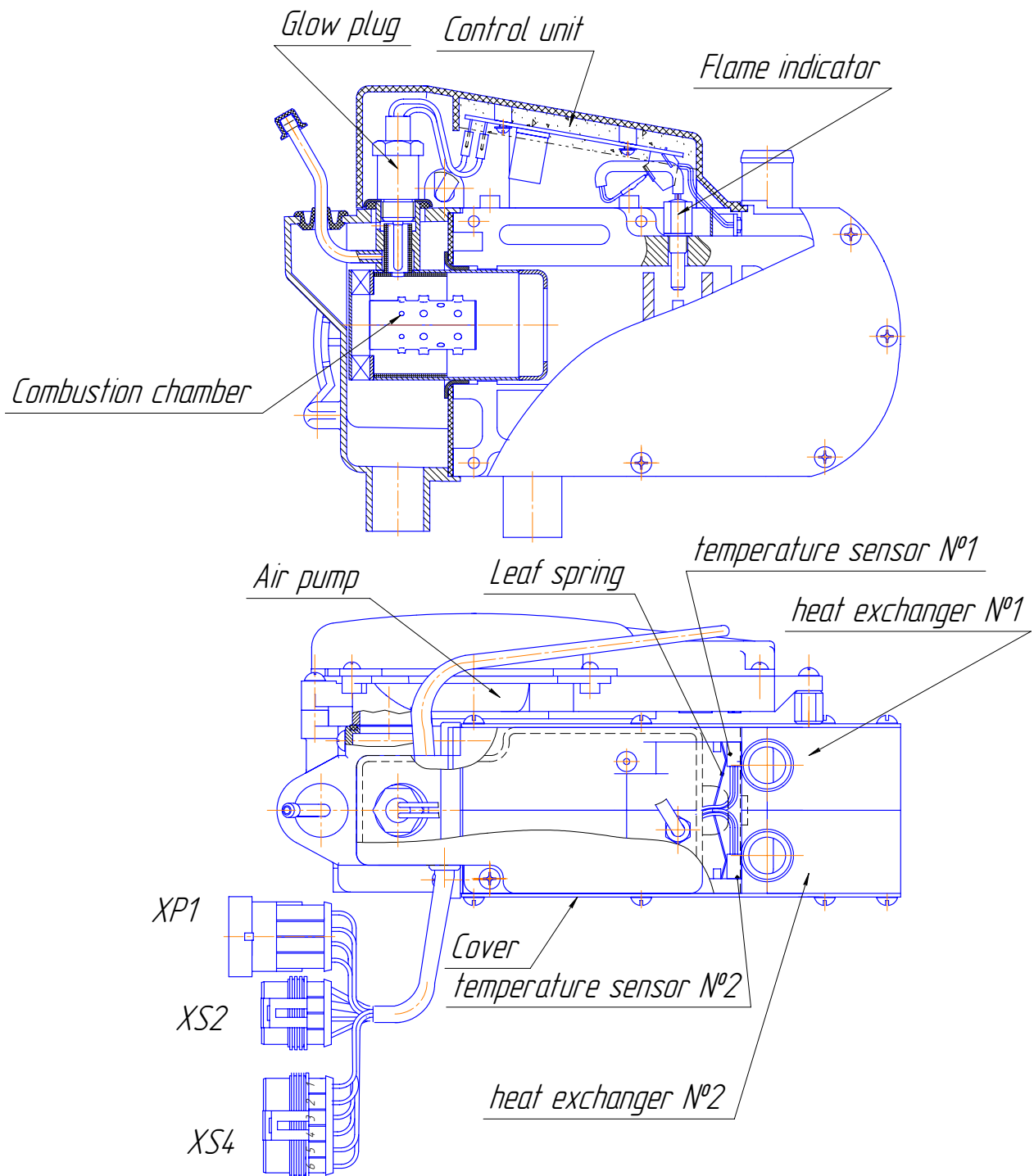
Figure 4.3 – Heater basic components
