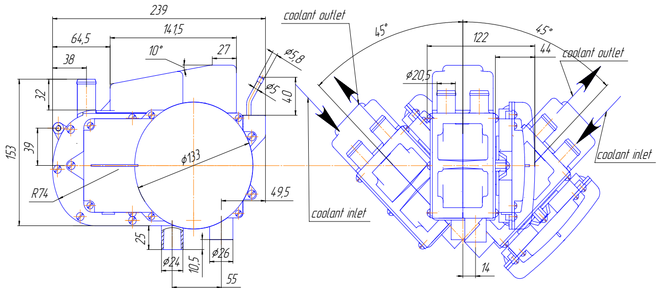
Figure 7.2 – Heater acceptable operating positions
