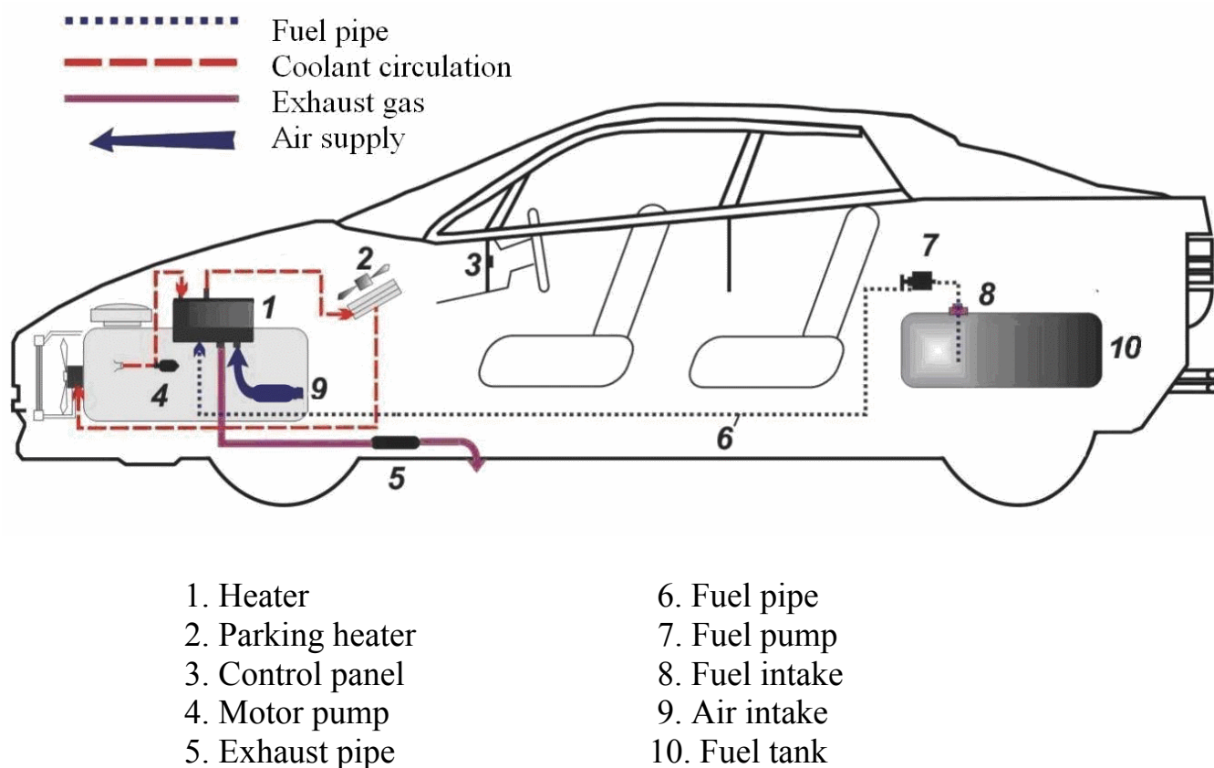
Figure 7.1 - Pre-heater installation diagram
