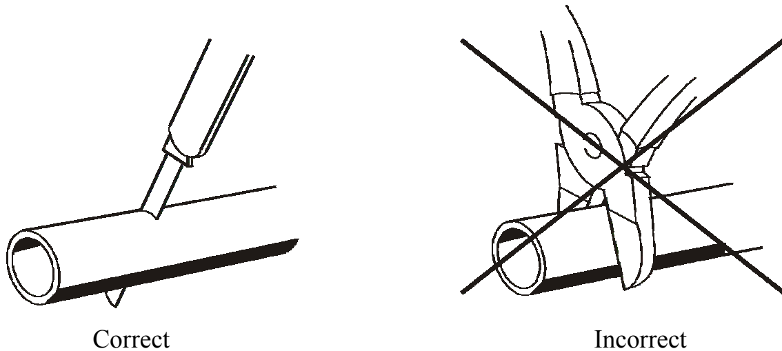
Figure 7.8 – Cutting the fuel pipe before installation
