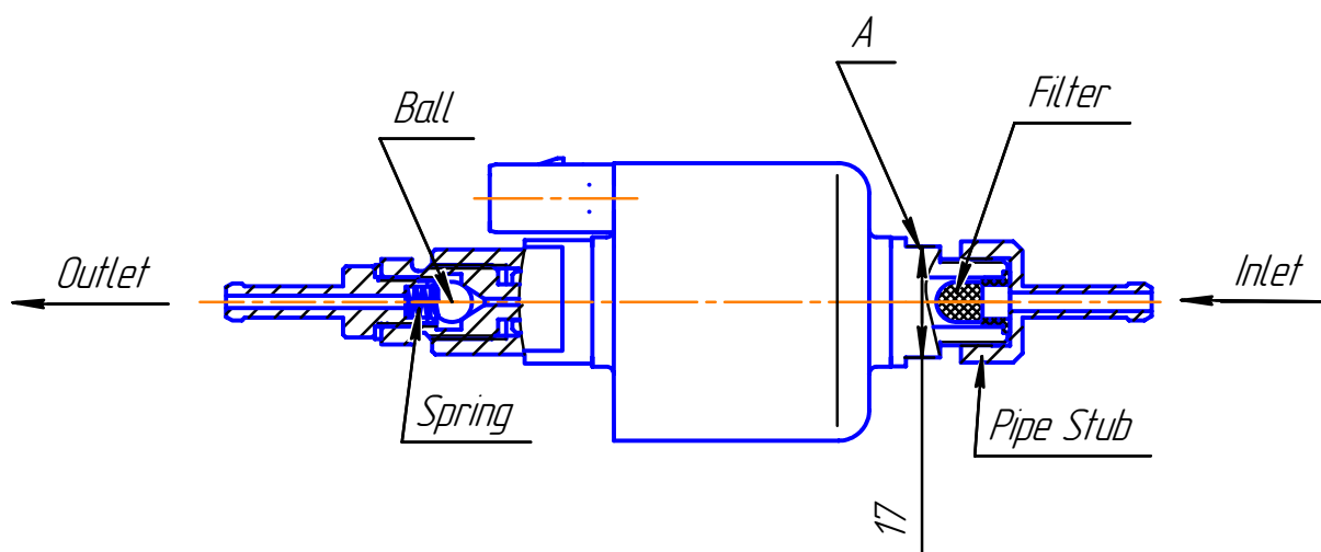
Figure 9.1 – Fuel pump
